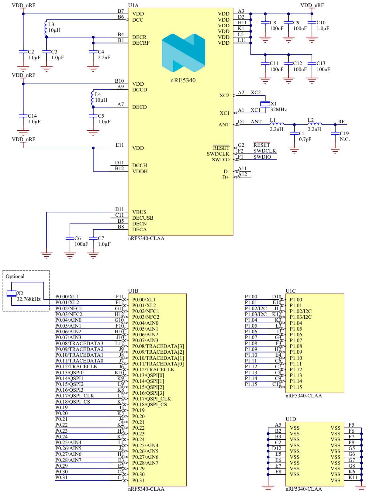
Figure 269: Circuit configuration no. 3 schematic
