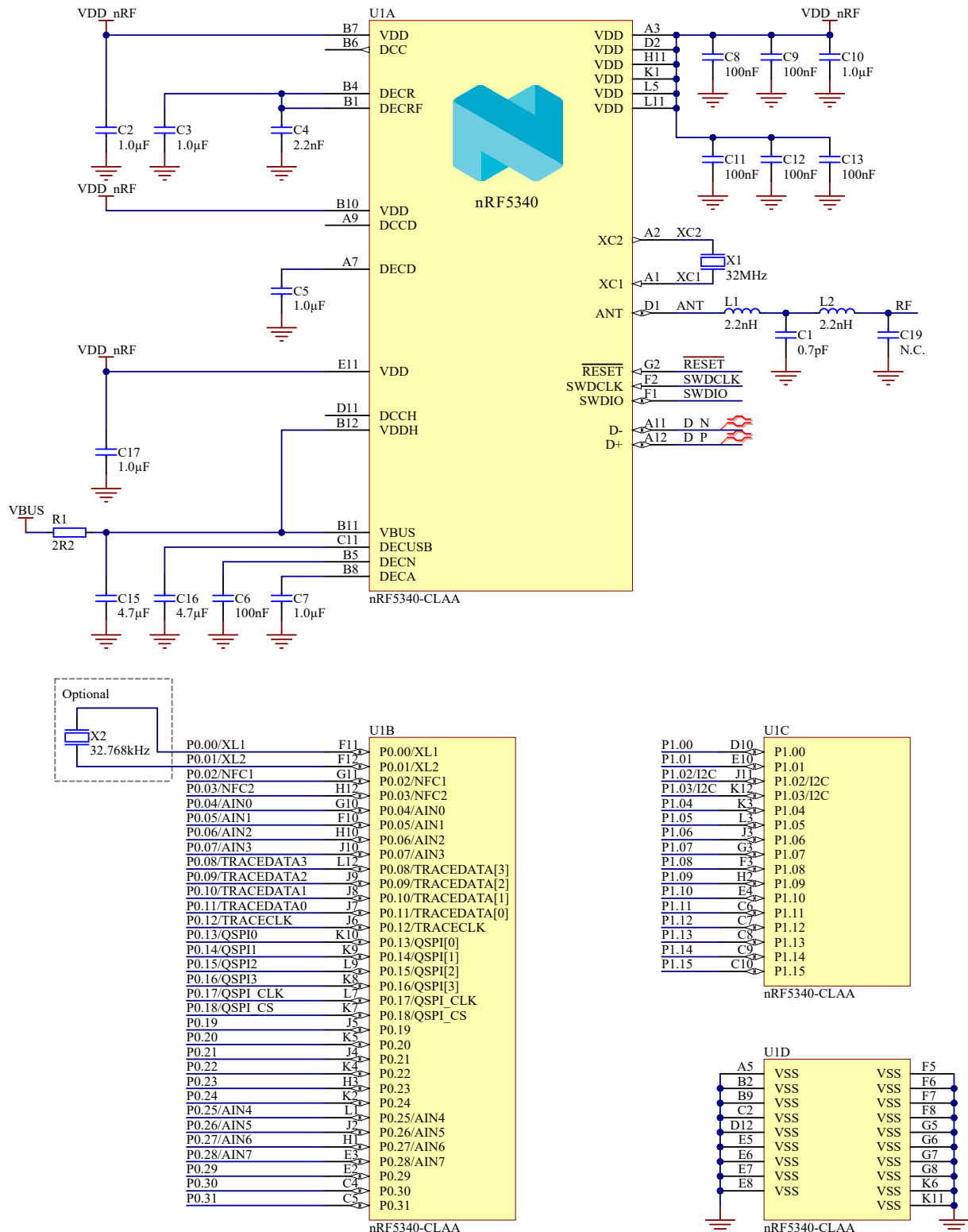
Figure 270: Circuit configuration no. 4 schematic
