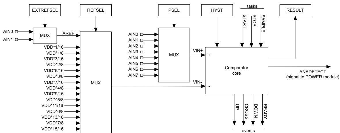
Figure 93: Low-power comparator
