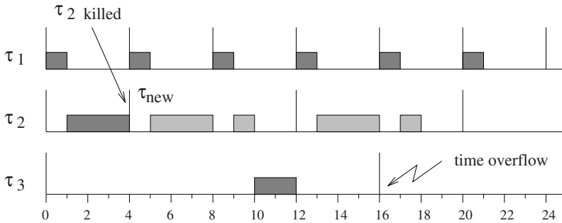
Figure 10.4 The effects of \tau_2 do not cancel at the time it is aborted, but protract till the end of its period.
