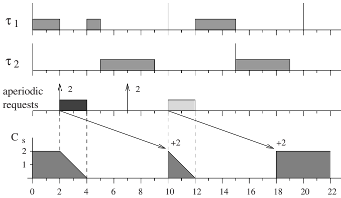
Figure 5.18 Example of a high-priority Sporadic Server.
